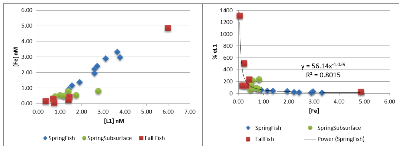
Fig. 3. A) The concentration of iron ([Fe]) relative to the concentration of the strong iron binding ligand class ([L 1 ]) shows L 1 was always in excess. B) The percentage of excess strong binding ligand concentration (% eL 1 ) relative to the concentration of dissolved iron ([Fe])
